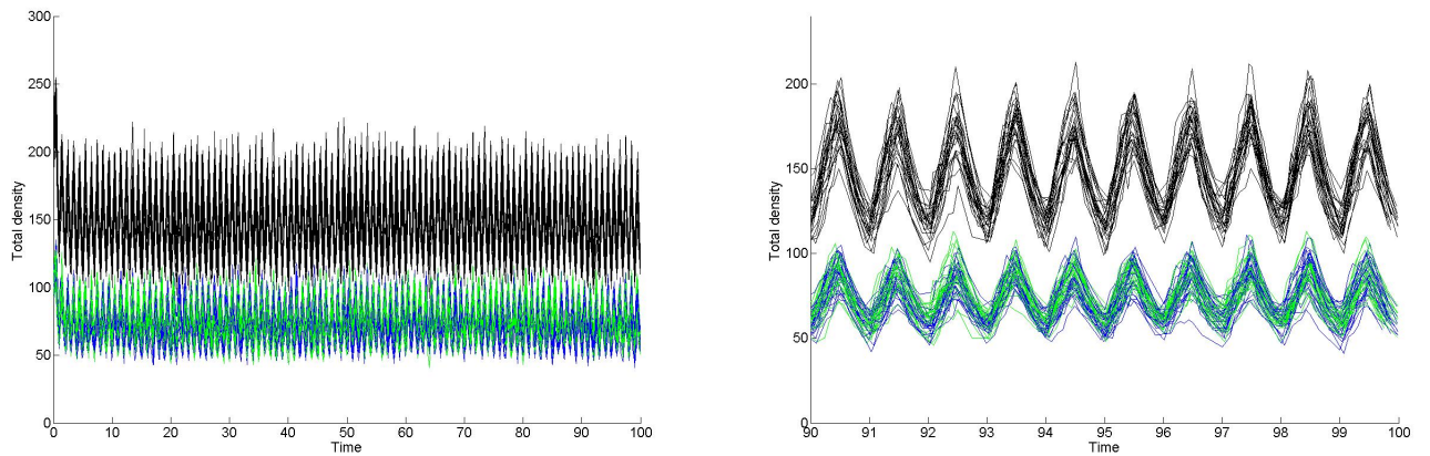
Figure 5: 25 model realisations using the high carrying capacity for 2012 in Kidland (blue), Uswayford (green) and both (black).
