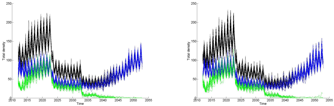
Figure 12: 50 model realisations when dispersal was prevented between Kidland/Tilhill and Uswayford (left) and when dispersal was allowed (right) in the high carrying capacity case for Scenario A for Kidland (blue), Uswayford (green) and both (black).
