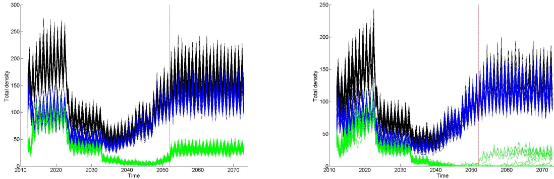
Figure 15: 50 runs with the high carrying capacities determined from Scenario A and global dispersal (left), 1km dispersal with connection (right) where the simulation are extrapolated for a further 20 year.
