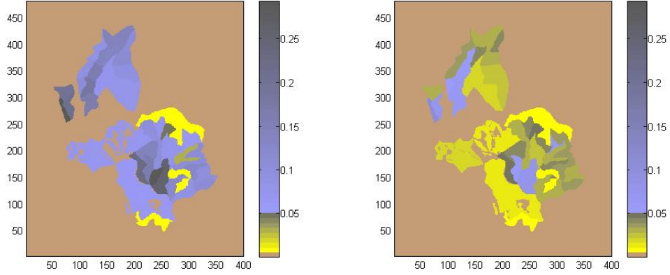
Figure 3: Red squirrel carrying capacities for Scenario A in 2012 for the high (left) and low (right) density estimates (units are squirrels per hectare).
