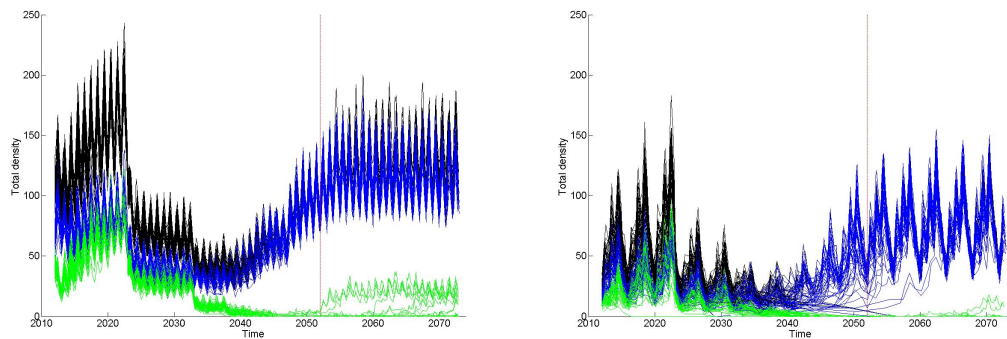
Figure 11: 50 model realisations with Scenario A's high carrying capacity (left) and 3 high, 1 low carrying capacity scenario (right) for 40 years with extrapolation of an additional 20 years beyond the red line in Kidland (blue), Uswayford (green) and both (black).
