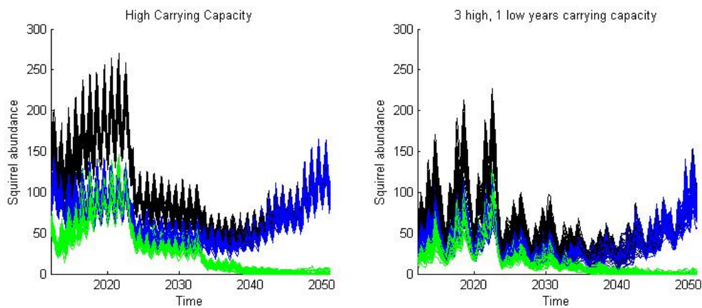
Figure 10: 50 model realisations for the high (left) and 3 high, 1 low (right) carrying capacity scenario driven by data derived by the original forest management plan (Scenario A) for 2012-2052 - Kidland (blue), Uswayford (green) and both (black).
