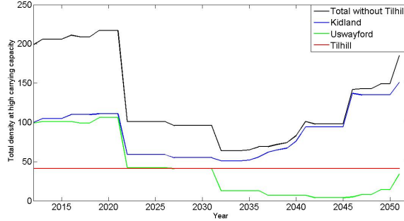
Figure 4: Changes in red squirrel carrying capacity using the high density estimates between 2012-2052 for Scenario A
