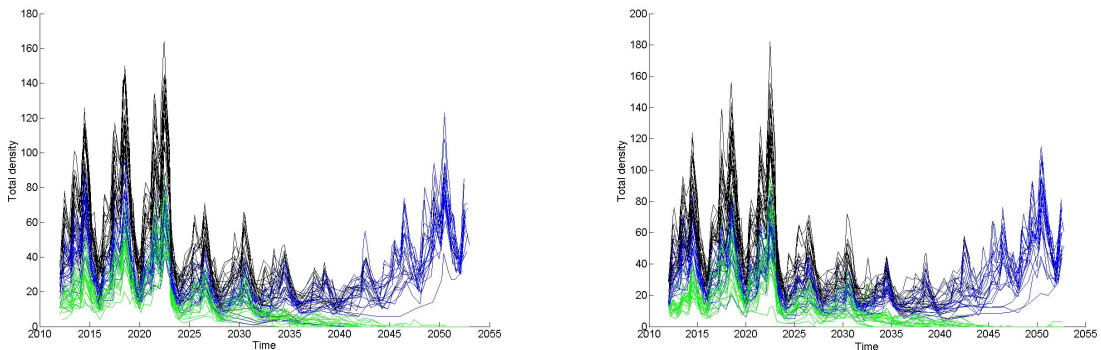
Figure 13: 50 model realisations when dispersal was prevented between Kidland/Tilhill and Uswayford (left) and when dispersal was allowed (right) in the 3 high, 1 low carrying capacity case for Scenario A for Kidland (blue), Uswayford (green) and both (black).
