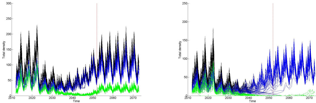
Figure 16: 50 runs with the 3 high, 1 low year carrying capacities determined from Scenario A and global dispersal (left), 1km dispersal with connection (right) where the simulation are extrapolated for a further 20 year.
