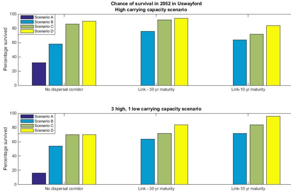
Figure 22: Percentage of survivals in Uswayford in 2052 for the four forest design scenarios where there is no dispersal corridor (left) and when the corridor is planted in the compartment shown in Figure 18 and has a 30 year growth time before it can be used (middle) or a 10 year growth time (right).
