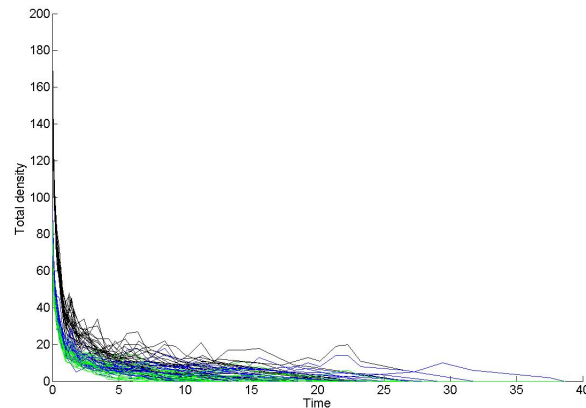
Figure 6: 25 model realisations using the low carrying capacity for 2012 in Kidland (blue), Uswayford (green) and both (black).
