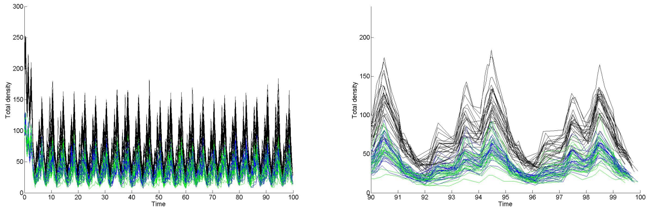
Figure 7: 25 model realisations using 3 good seed years followed by 1 poor year for 2012 in Kidland (blue), Uswayford (green) and both (black)
